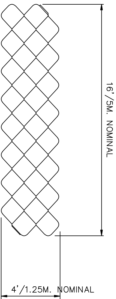
PLAN VIEW
